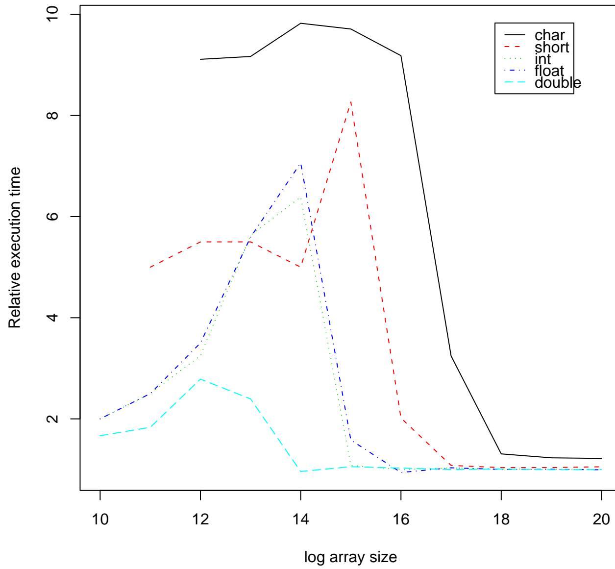
Relative execution time for char, short, int, float and double arrays
